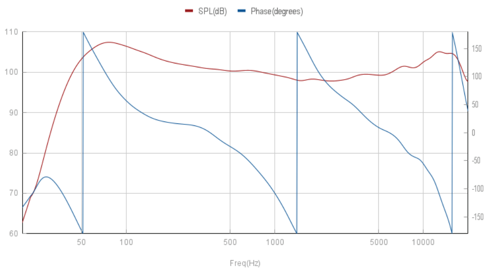
Frequency & Phase Response - Processed
