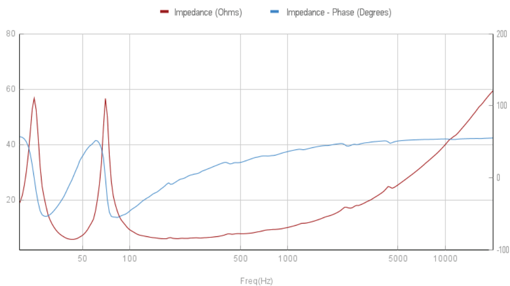
LF Impedance & Phase Response
