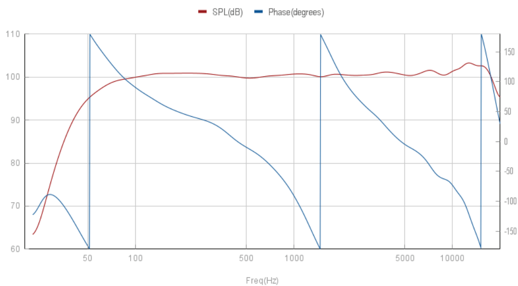
Atomik Epoch -1 - Frequency & Phase Response - Flat
