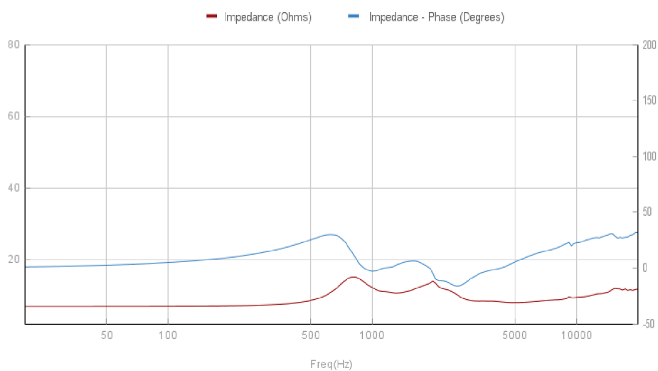
HF Impedance & Phase Response
